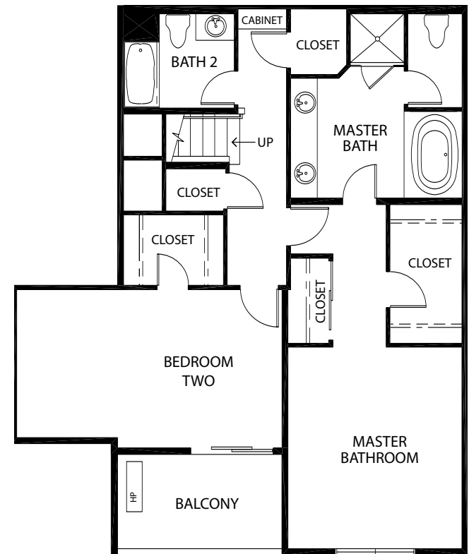
Lower Floor
